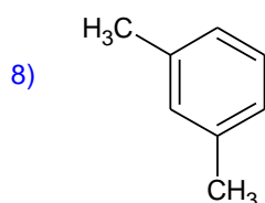
m-xylen 1,3-dimethylbenzen
