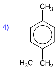
4-ethyltoluen 1-ethyl-4-methylbenzen
