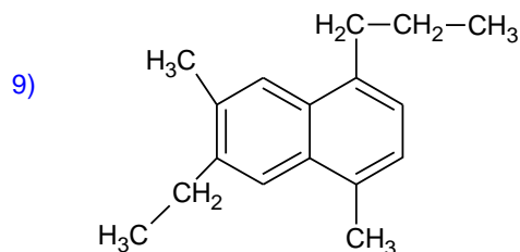
6-ethyl-4,7-dimethyl-1-propylnaftalen
