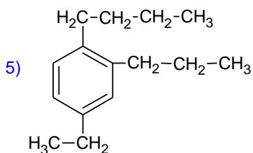
1-butyl-4-ethyl-2-propylbenzen
